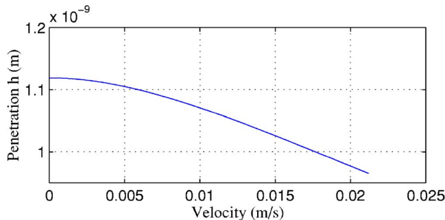
Fig. 13 Computed COF for a larger velocity range
