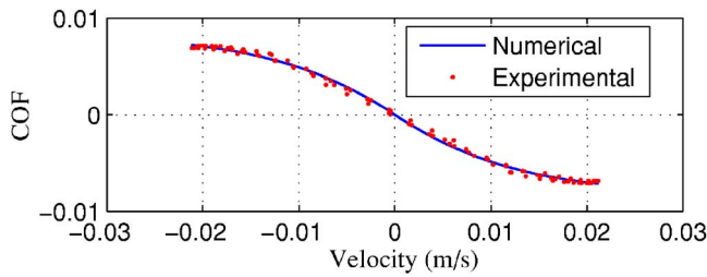
Fig. 12 Computed COF versus experimental measurement
