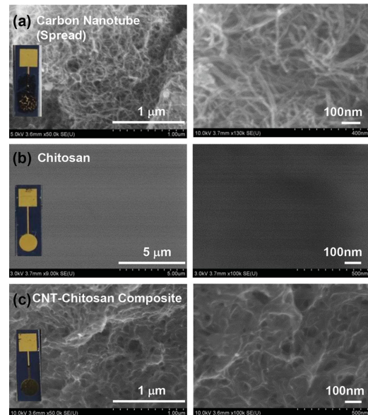
Figure 3. Scanning electron microscope (SEM) characterization. a) Spread CNT. b) Electrodeposited chitosan film. c) Electrodeposited CNT-chitosan composite film.
