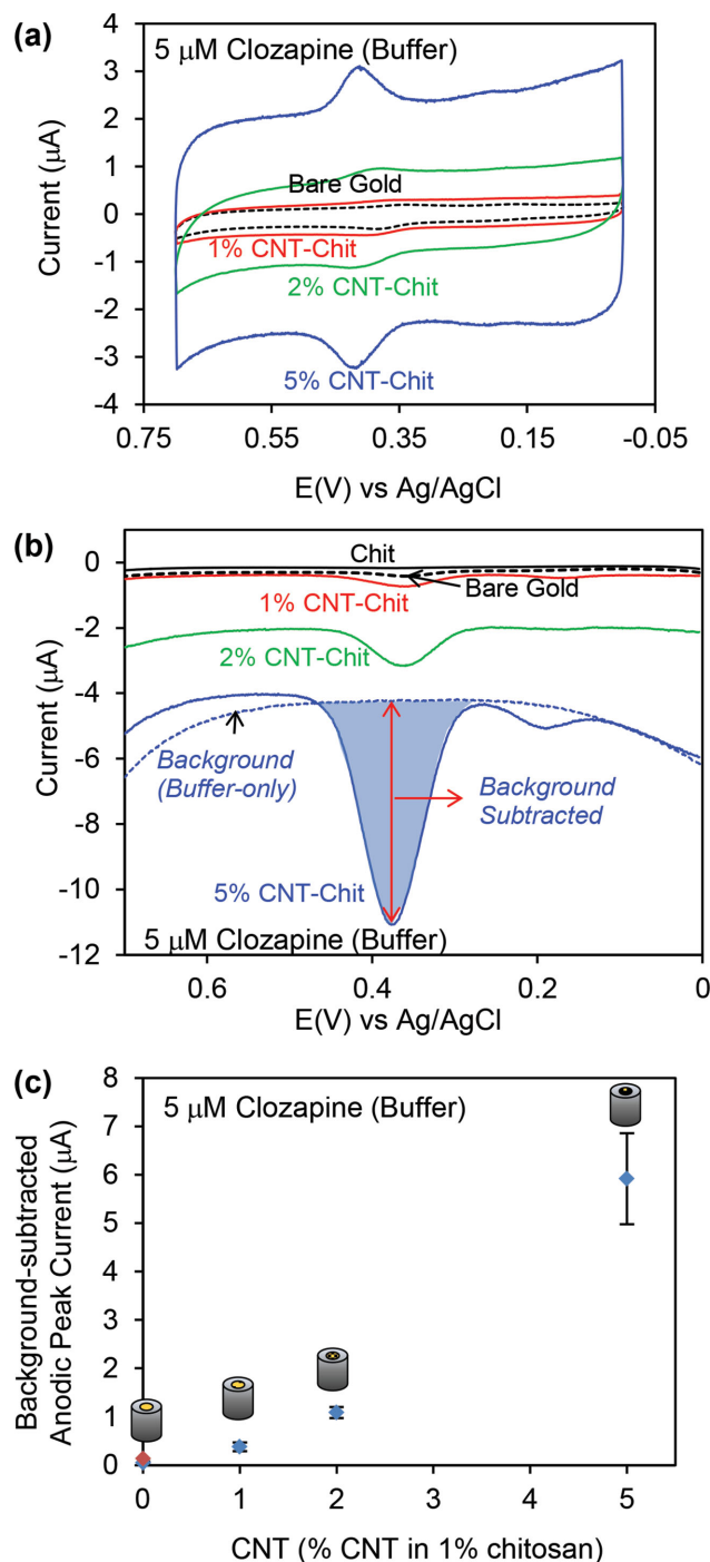
Figure 5. Carbon nanotubes (CNTs) enhance the electrochemical oxidation of clozapine ( 5 \times 10^{-6}\text{ M} ). a) Cyclic voltammograms (CVs). b) Differential pulse voltammograms (DPVs). c) Plot of anodic peak current (DPV) versus CNT content in the deposition solution. Analysis performed in 0.1\text{ M} phosphate buffer (pH 7).
